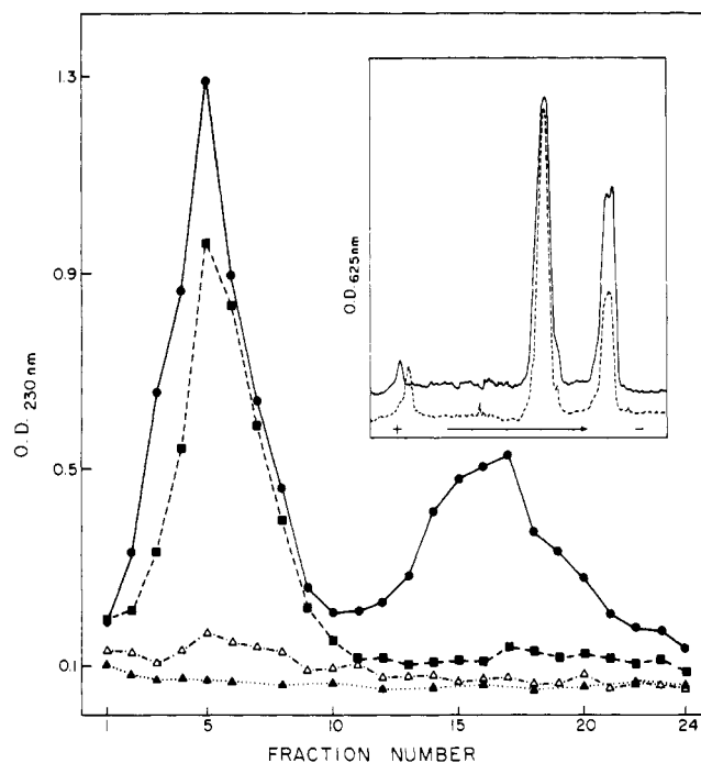
FIGURE 3: Sucrose gradient centrifugation profiles of histone preparations and their mixtures. The amount of each histone applied to a single gradient was as follows: 270 \mu g of f2a1 ( \Delta — \Delta ); 290 \mu g of f3 ( \square — \square ); 231 \mu g of f2a1 + 553 \mu g of f3 ( \square — \square ); 231 \mu g of f2a1 + 553 \mu g of f3 + 297 \mu g of f1 ( \bullet — \bullet ). Inset: Densitometer tracings of polyacrylamide gel electrophoresis. Fractions 2–9 from each sucrose gradient were pooled, concentrated, and analyzed by gel electrophoresis. The tracings show the analyses from the gradient in which both f3 and f2a1 were applied (—) and the gradient in which f3, f2a1, and f1 were applied (—). Direction of protein migration is indicated by the arrow. Viewing the inset from right to left, the two main peaks correspond to histones f2a1 and f3, and the small peak on the far left corresponds to a polymerized form of f3.
