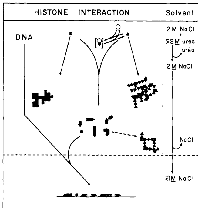
FIGURE 7: Working model which proposes the histone interactions involved in the binding of f3 and f2a1 to DNA. The monomers are represented as follows: f3 ( \boxtimes ), f2a1 ( \blacktriangle ), f1 ( \circ ). In the presence of 2 M NaCl and 2 M urea no stable interactions may exist between histones or between histones and DNA. After removal of urea, but still in high salt, most of histone f3 aggregates in complexes of varying size, as does all of histone f2a1 separately. As the salt concentration is decreased, another type of interaction begins to take place, i.e., the formation of f3-f2a1 complexes whose stoichiometry is dependent on the relative concentration of the proteins. In low ionic strength these complexes, as well as some free f3, can bind to DNA.
