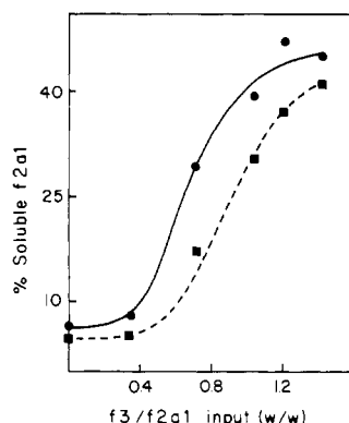
FIGURE 4: Effect of f3 on the solubility of [ ^{14}\text{C} ]cyanamide-f2a1 in the presence of f1 (●—●) and in the absence of f1 (■—■). The f2a1 concentration was 50 \mu\text{g}/\text{ml} and the f1 concentration was 59 \mu\text{g}/\text{ml} .
